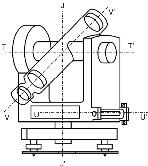
36- rasm. Teodolitning asosiy geometrik o‘qlari: JJ\bigtriangledown — asbobning aylanish o‘qi; TT\bigtriangledown — ko‘rish trubasi aylanish o‘qi; UU\bigtriangledown — silindrik adilak o‘qi.
