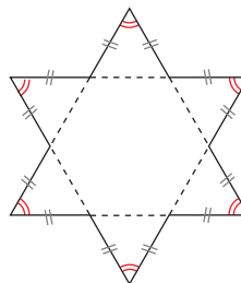
Hexagram
