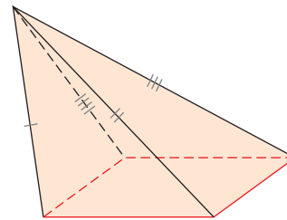
Square pyramid (b)
