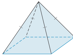
Regular square pyramid (a)
