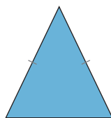
Isosceles Triangle
