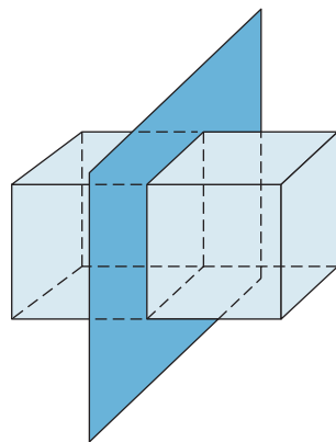
Right rectangular prism
