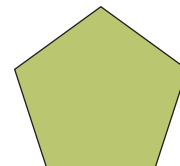
Regular Pentagon
