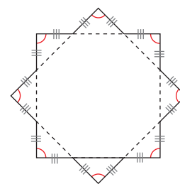
Octagram
