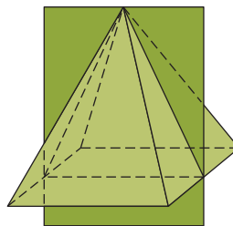
Regular square pyramid
