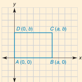
Rectangle
