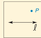
(a) Small part of surface of the sphere
