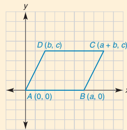
Parallelogram
