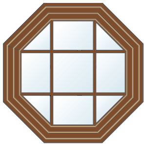
The four triangular panes in the octagonal window are congruent triangles.
