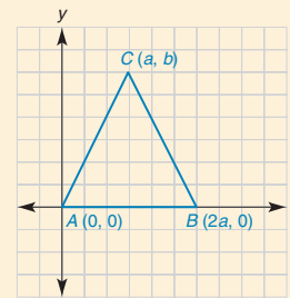
Isosceles Triangle
