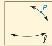
(b) Line through P “parallel” to \ell on larger part of surface
