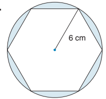
Regular hexagon inscribed in a circle
