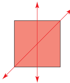
Square
