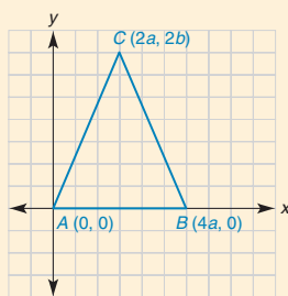
Isosceles Triangle (Midpoints)
