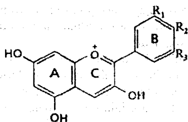
Antostionidin
