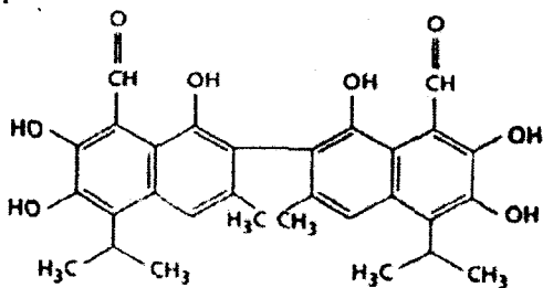
Gossipol
