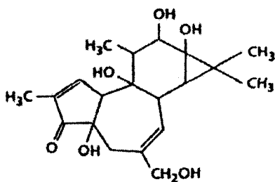
Forbol
