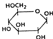
\beta -D-glyukoza
