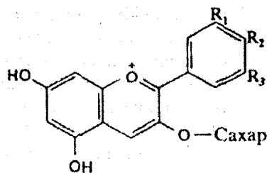
Antostionidinni tuzilishi
